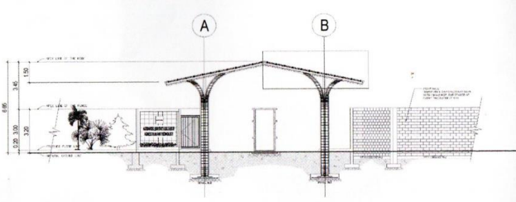
2 SECTION THRU A-A S-2 SCALE 1/8"
