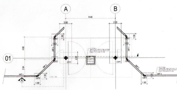
1 FOUNDATION PLAN S-2 SCALE 1/16"
