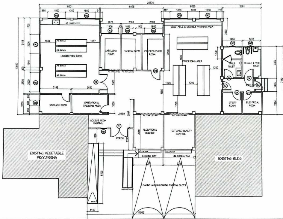
R R O W ○ FLOOR PLAN SCALE: 1:100 MTS
