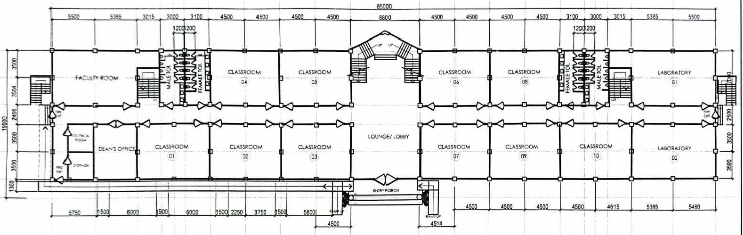
GROUND FLOOR PLAN SCALE: 500 IMTS
