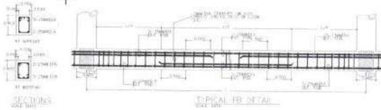
TYPICAL TIE BEAM
