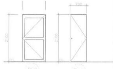
28 UNITS 1.00 X 2.10 SLIDING DOOR WITH 6MM THICK COLORED GLASS ON TUBULAR ALUMINUM FRAME 8 UNITS HOLLOW CORE FLUSH TYPE DOOR ON 70x150mm THICK COLORED GLASS ON WOODEN JAMBS/FRAMES W/ COMPLETE ACCESSORIES.
