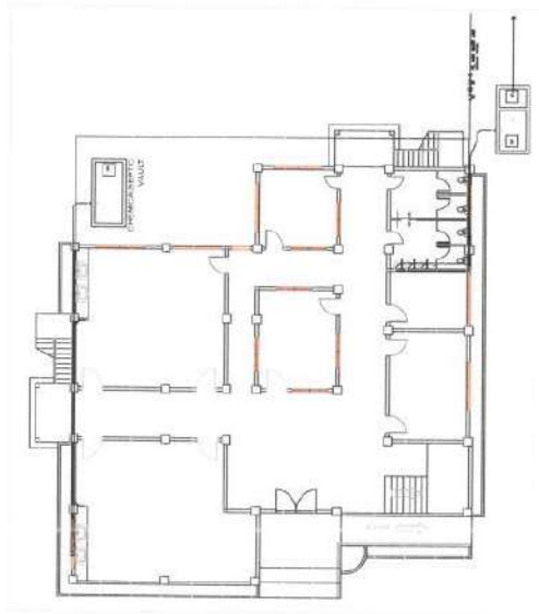
FIRST FLOOR PLUMBING LAYOUT
