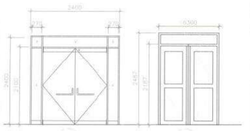
1-0.75 X 2.10 DOUBLE SWING DOOR WITH 6MM THICK COLORED GLASS ON TUBULAR ALUMINUM FRAME 4-0.75 X 2.10 DOUBLE SWING DOOR WITH 6MM THICK COLORED GLASS ON TUBULAR ALUMINUM FRAME
