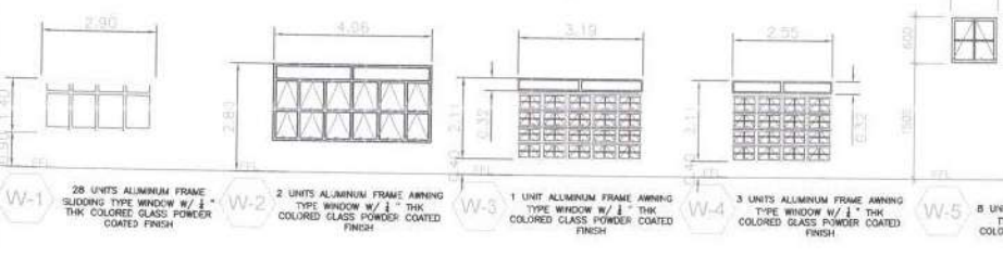
WINDOWS DETAILS
