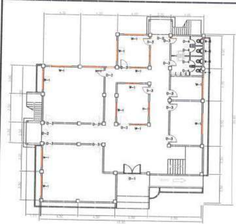
FIRST FLOOR DOOR AND WINDOW SCHEDULES
