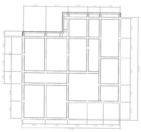
ROOF BEAM PLAN
