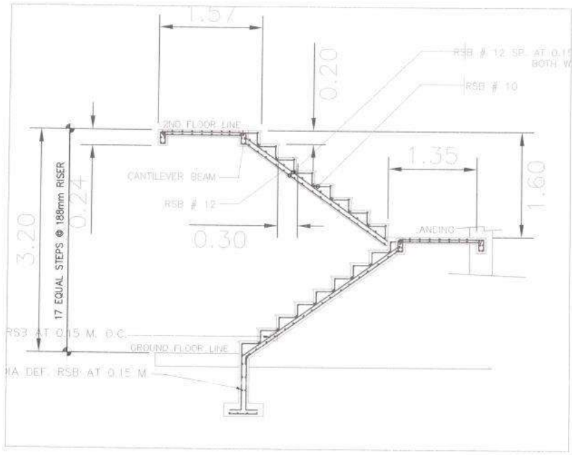
STAIR DETAILS
