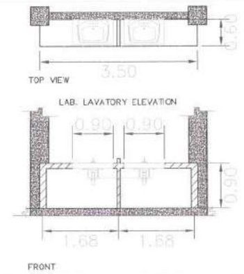
FRONT
