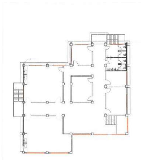
SECOND FLOOR PLUMBING LAYOUT
