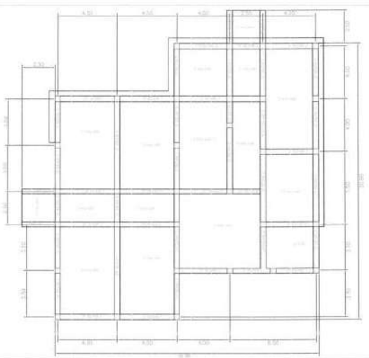
SECOND FLOOR BEAM PLAN
