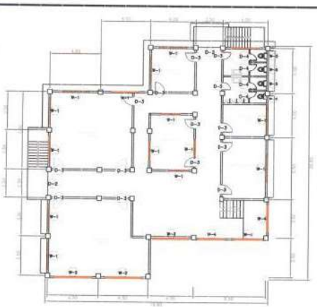
SECOND FLOOR DOOR AND WINDOW SCHEDULES
