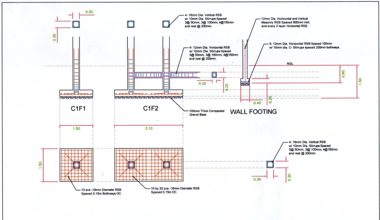
STAGE FOOTING, COLUMN, TIE BEAM AND WALL FOOTING PLAN
