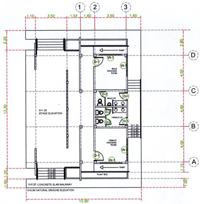
STAGE FLOOR PLAN
